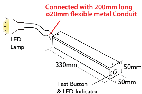
LED Lamp Dimension: ø85mm Ceiling Cutout: ø75mm
